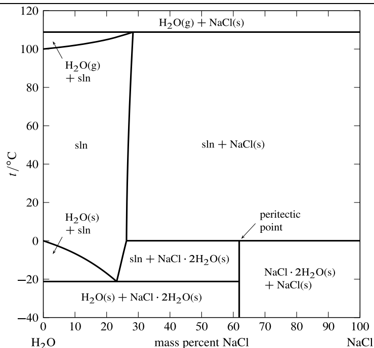
Figure 13.2.4. Temperature--composition phase diagram for the binary system of \text{H}_2\text{O} and \text{NaCl} at 1 bar. (Data from Refs. [37] and [181].)
